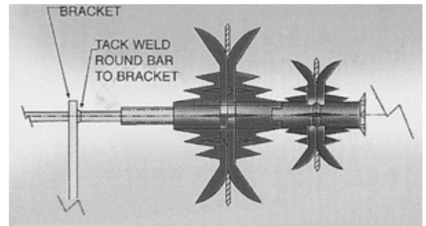
Spinner mounting detail.
