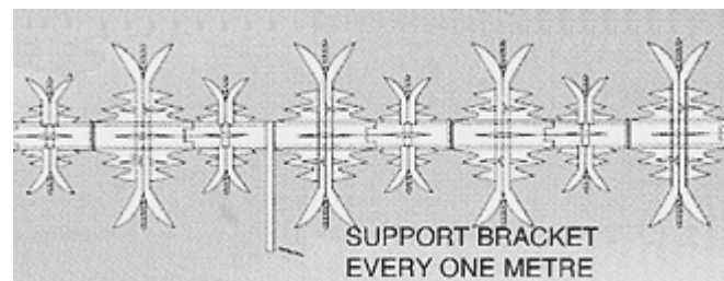
General arrangement of spinner installation.
